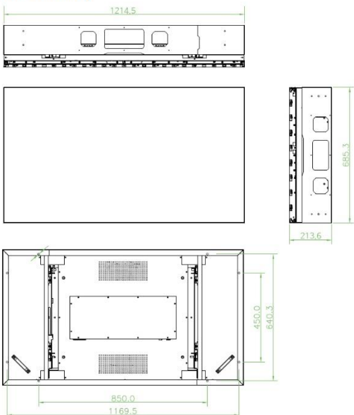
[Outside Dimension]
